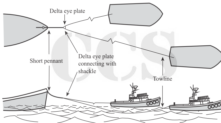
Figure 1.4 Diagram of multiple tugs to one tow
